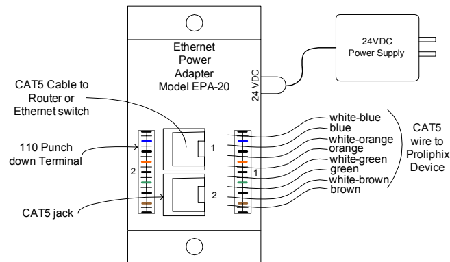
Figure 1 EPA-20 Wiring
