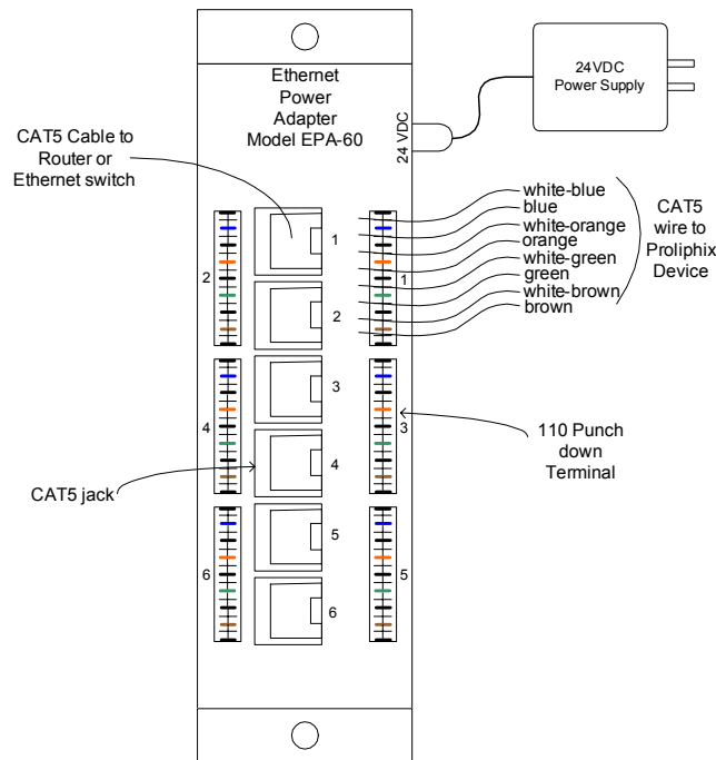
Figure 2 EPA-60 Wiring
